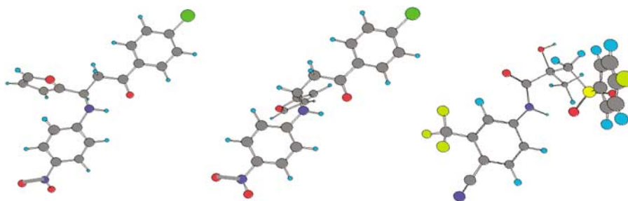
Figure 5 Three dimensional structures of the two enantiomers of compound 21 (left and middle panel) and Casodex (right panel).
